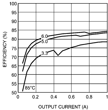
Efficiency 42V Input @ 85°C
