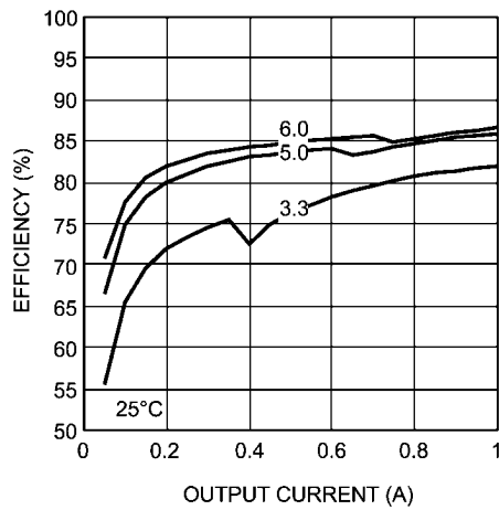
Efficiency 36V Input @ 25°C
